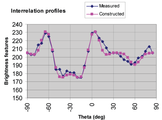
Fig. 4: Measured and reconstructed interrelation profiles
