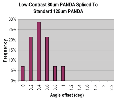
Fig. 5: LC 80 \mu m PANDA to 125um PANDA
