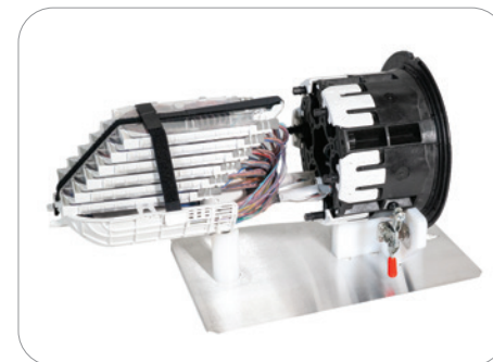
Apex X-2S Mounted on Installation Stand
