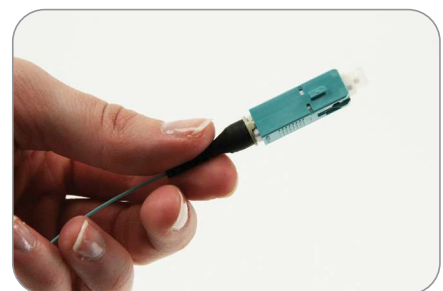
6—Apply housing, boot and dust cap
