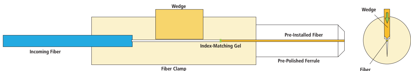
Figure 1—FASTConnect SC, LC and ST Connectors
