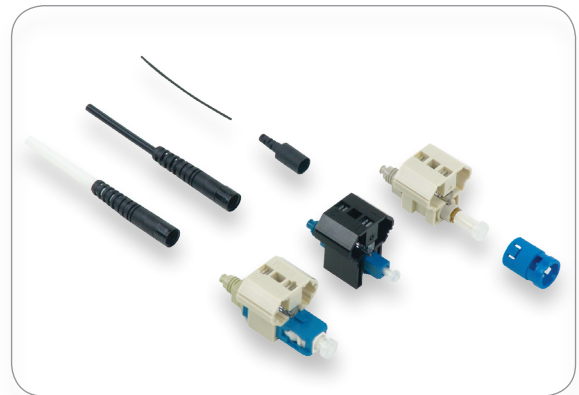
Figure 1—FASTConnect SC, LC and ST Connectors
