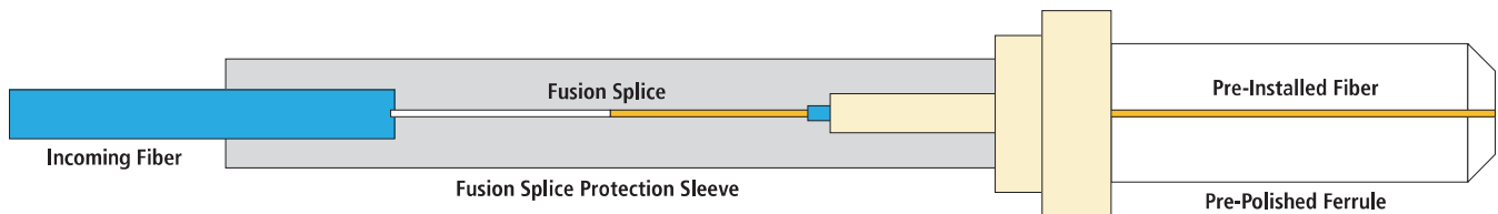
Figure 2—FUSEConnect SC, LC and ST Connectors
