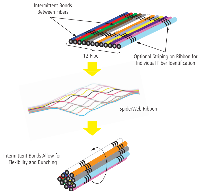
Figure 1—SpiderWeb Ribbon Design and Functionality
