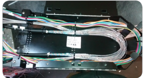
Photograph 4—Network Splice Organizer 432F WTC and 144F Loose Tube Cables
