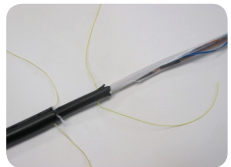
Photograph 12—WTC Inner and Outer Ripcords
