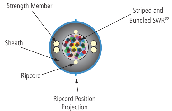
Figure 2—Wrapping Tube Cable Cross-Sectional View
