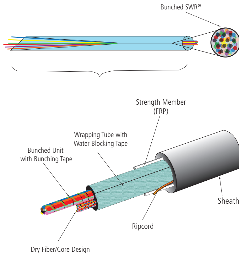
Figure 3—Wrapping Tube Cable Detailed Assembly View
