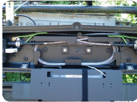
Photograph 10—Aerial Breathable Access Closure WTC Storage
