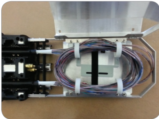
Photograph 7—WTC 576F Storage in Sealed Access Closure
