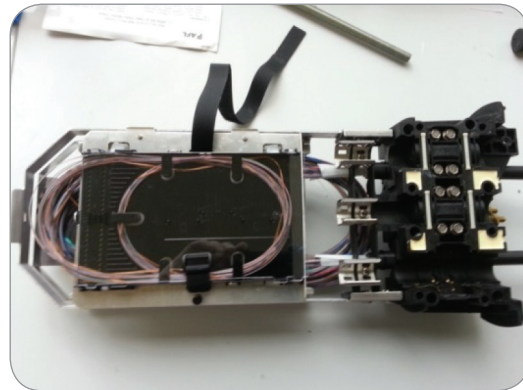
Photograph 8—WTC 144F Sealed Access Splice Tray
