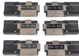
900 µm, 250 µm, 12F Ribbon Fiber Holders
