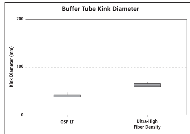
Figure 6—Buffer Tube Kink Diameter Comparison
