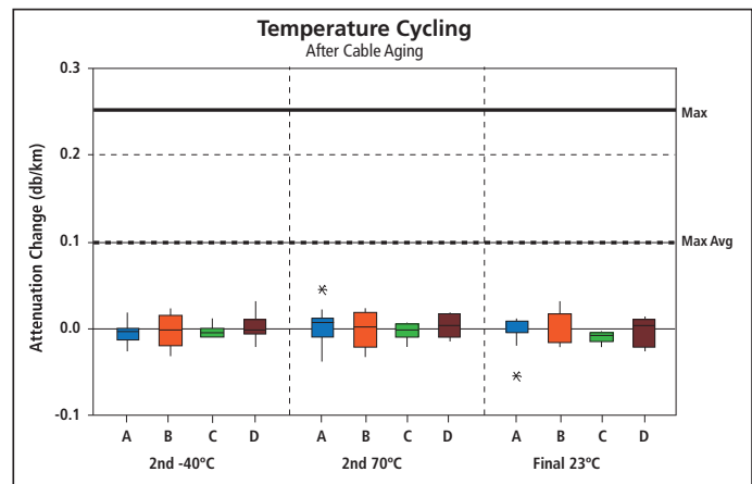
Figure 8—Cable Temperature Cycling after Cable Aging
