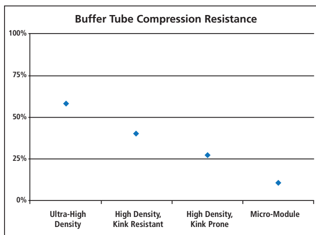
Figure 4—Buffer Tube Compression Resistance
