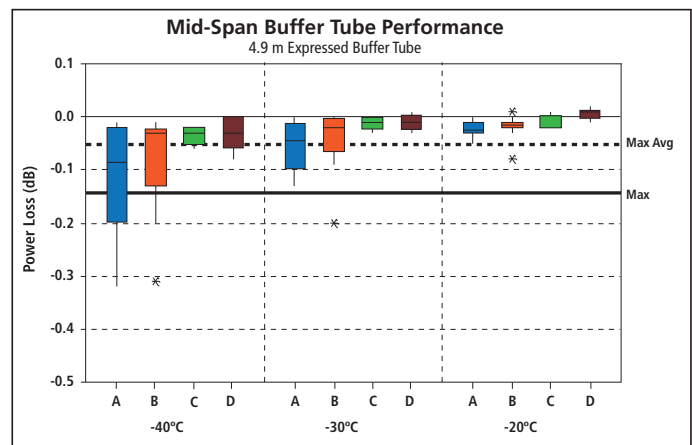
Figure 10—Mid-Span Buffer Tube Performance
