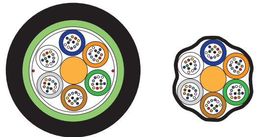
Figure 2—OSP Cables with 72 Fibers
