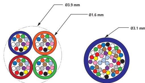
Figure 3—Micro-Modules vs. Ultra-High Fiber Density Buffer Tube
