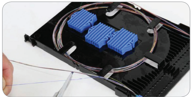
Figure 16—Fiber Bundle Storage and Fiber Access
