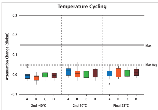
Figure 7—Cable Temperature Cycling
