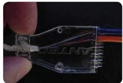
Figure 17— Fiber Routing and End Access
